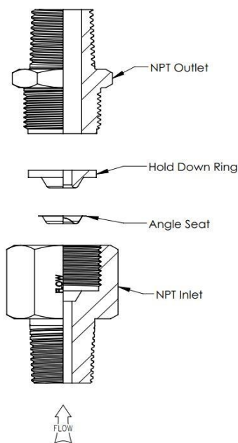
Figure 3 – Angle Seated Disk Screw Type Holder
