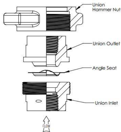
Figure 3 – Angle Seated Disk w/ Hammer Nut Union Type Holder
