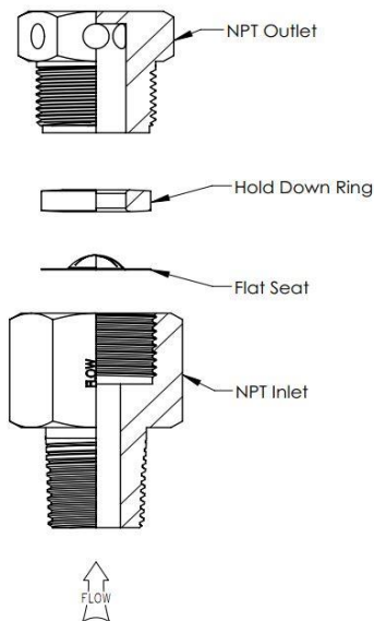
Figure 4 – Flat Seated Disk Screw Type Holder
